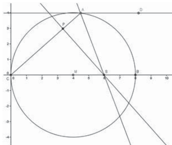
Figure 1. Translating the definition of Schmidt to the DGS
