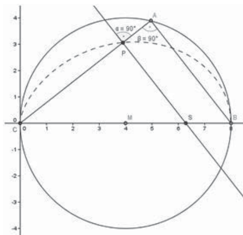
Figure 4. Affinity of the triangles
