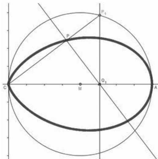
Figure 6. Egg-curve construed by DGS
