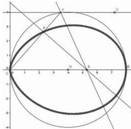
Figure 2. Egg-curve construed by DGS
