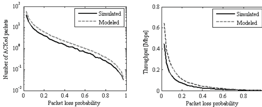
Figure 4. Simulation results: ns2 parameters: link speed 10Mbps, link delay 25ms, packet size 1024B, number of packet acknowledge by one ACK set to 1.
