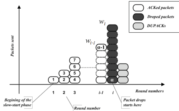
Figure 1. Slow-start phase, packet drop occurred at beginning of the round i
