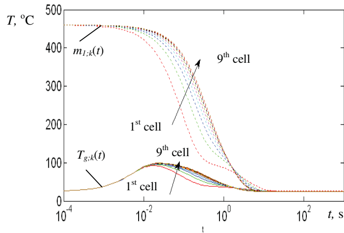
Figure 4: Transients of the mean temperature of particles and the temperature of air in the cells
