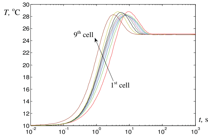
Figure 5: Transients of the temperature of water flowing in the tube
