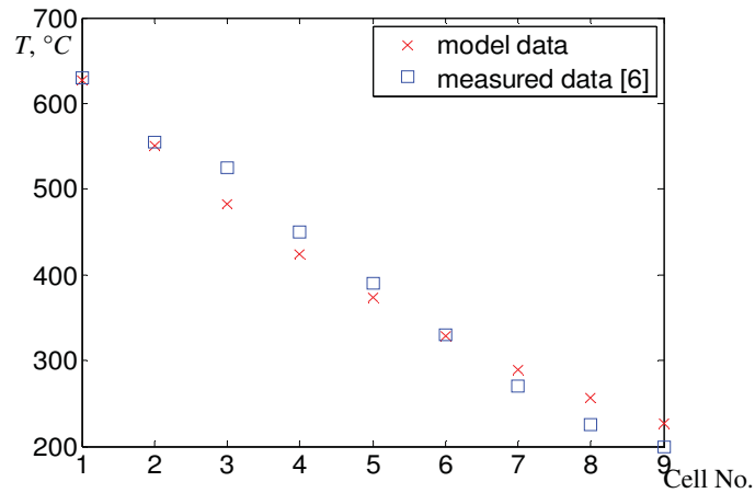
Figure 3: The results of the compartment/population balance model compared with the experimental data by Pécora and Parise [6]
