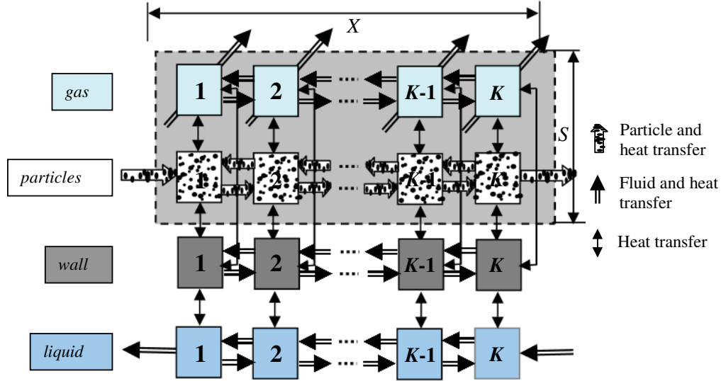
Figure 1. The scheme of the system
