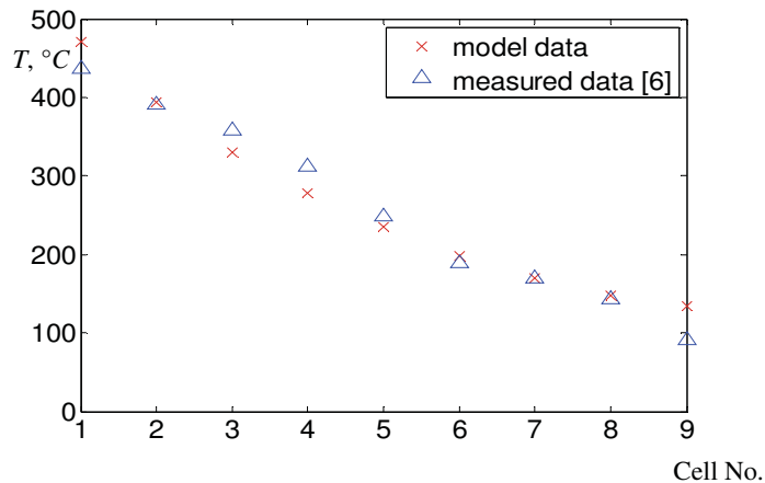
Figure 2: The results of the compartment/population balance model compared with the experimental data by Pécora and Parise [6]
