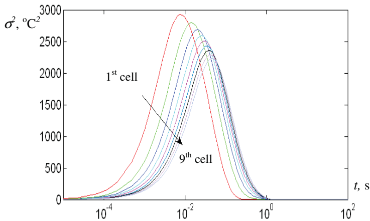
Figure 6: Transients of the variance of temperature of particle population
