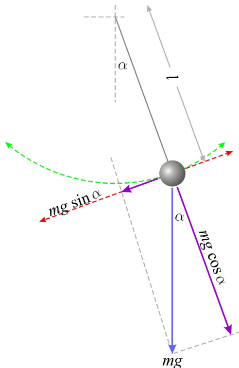
Fig. 1 Force diagram of a simple gravity pendulum
