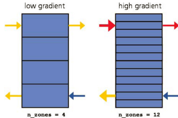
Fig. 2 Structural variable storage model, which uses a different number of zones in dependency of the current thermal layering
