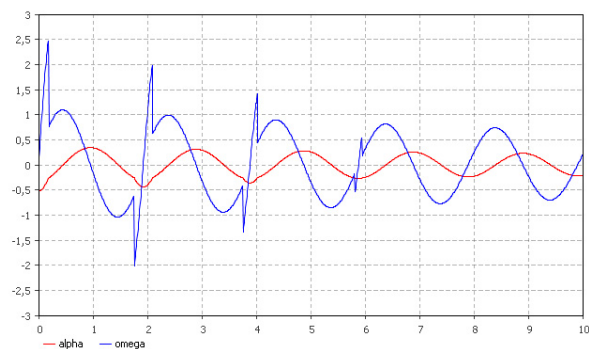
Fig. 7 The angle (red) and the angular velocity (blue) of the constrained pendulum (example 2)
