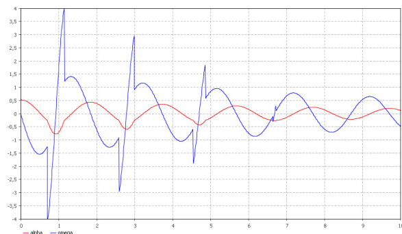
Fig. 6 The angle (red) and the angular velocity (blue) of the constrained pendulum (example 1)
